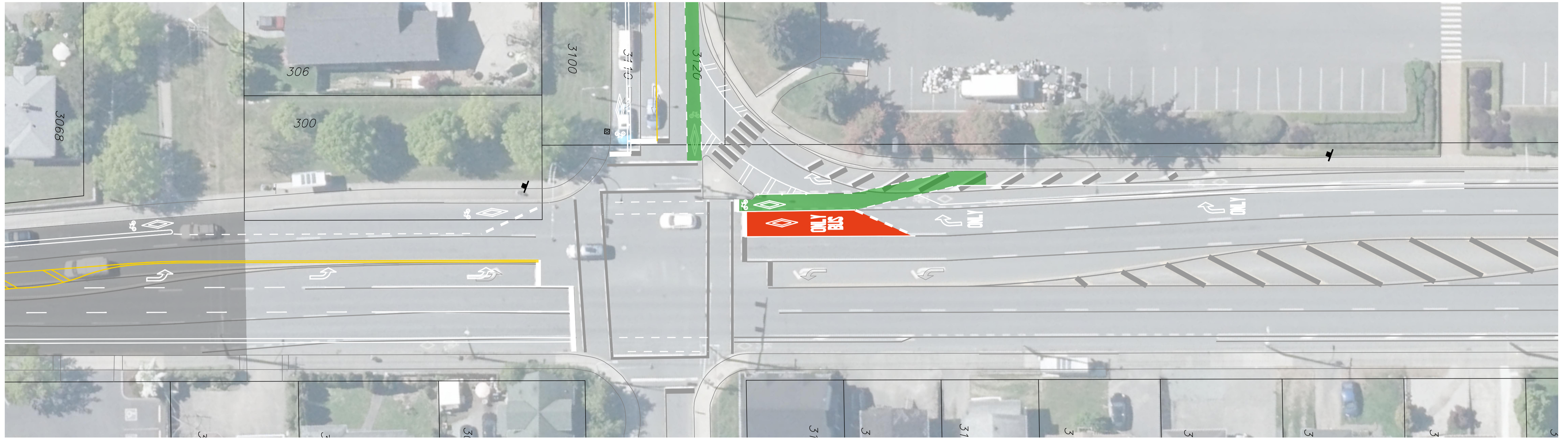
TILlicum QUICK BUILD - KERR AVE TO ARENA WAY SCALE H 1:250
