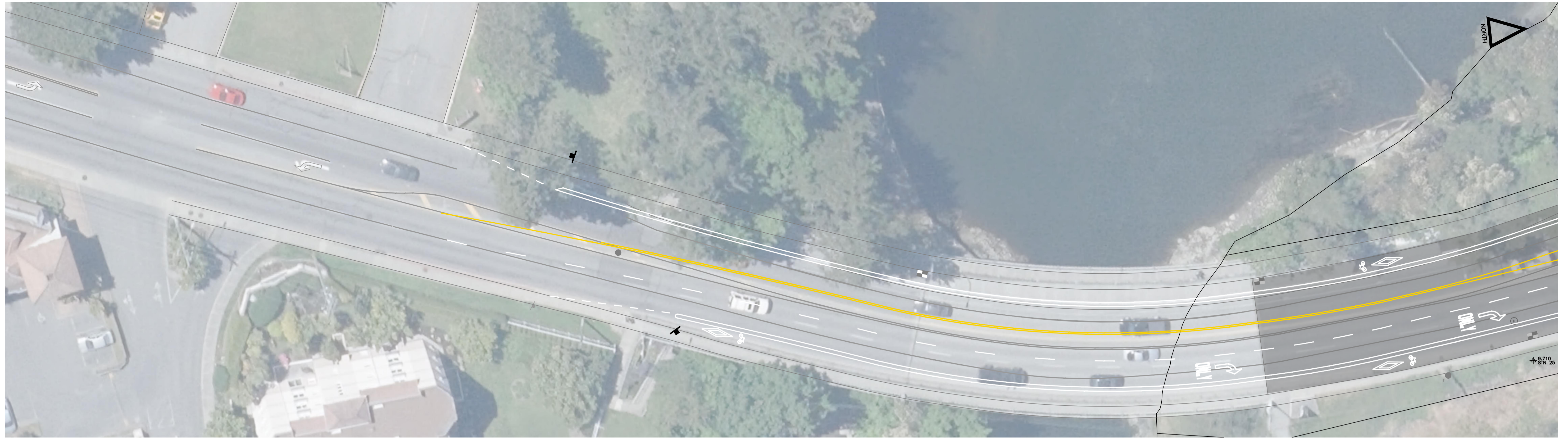
ESQUIMALT BORDER TO GORGE ROAD SCALE H 1:250
