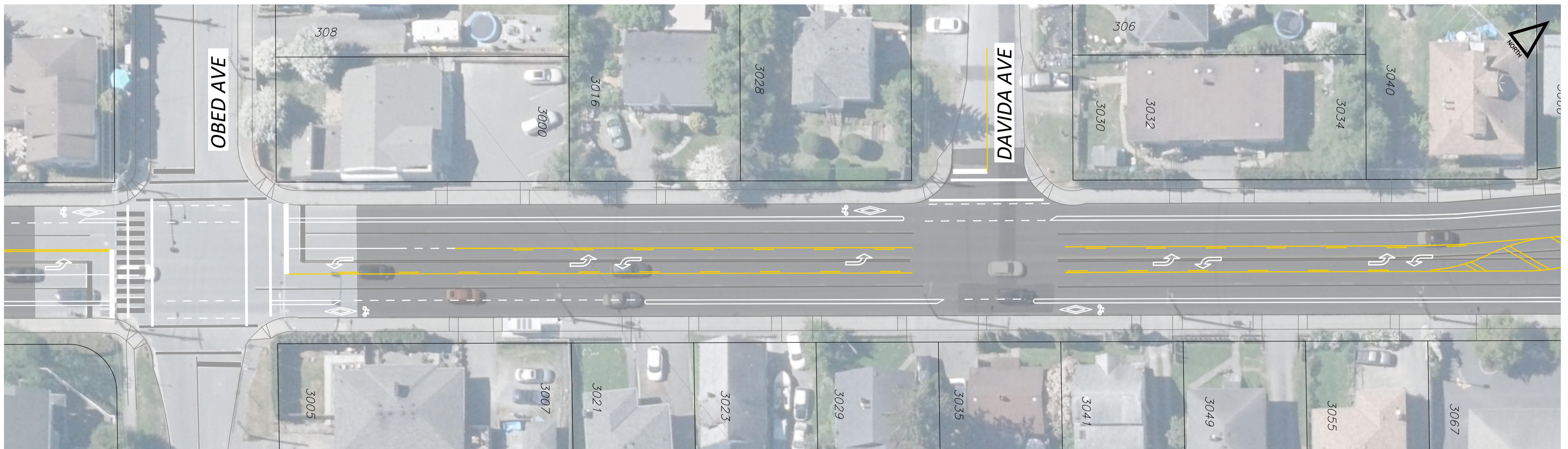
TILLICUM QUICK BUILD - WALTER AVE TO DAVIDA AVE SCALE H 1:250
