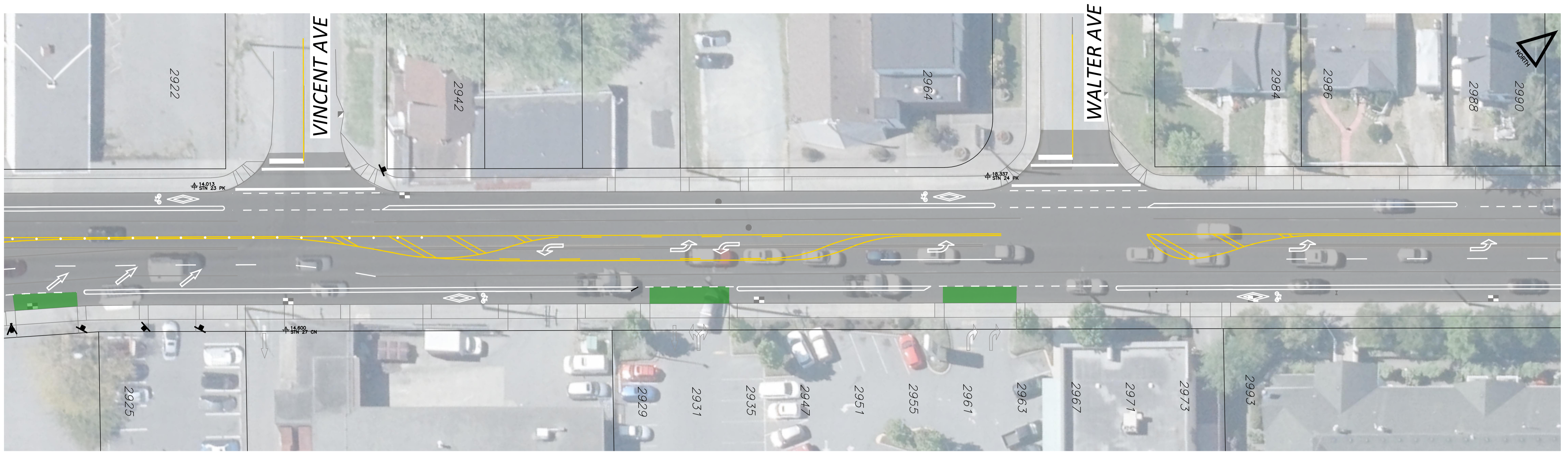
TILLICUM QUICK BUILD - ARNOT AVE TO WALTER AVE SCALE H 1:250
